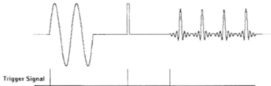
Figure 3-7, Sequenced Waveforms – Triggered Advance Mode
