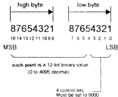
Figure 3-2, 12-Bit Waveform Data Format
