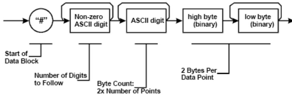
Figure 3-1, Definite Length Arbitrary Block Data Format
