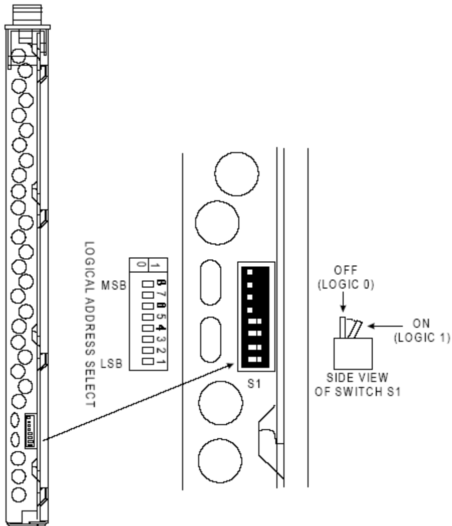
Figure 2-1, Set the Logical Address
