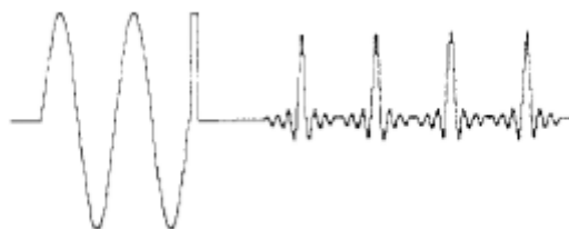
Figure 3-6, Sequenced Waveforms – Continuous Advance Mode
